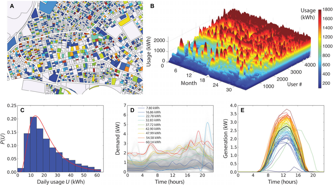
Fig. 1. (A) Map of a portion of Cambridge, MA. The colors represent the monthly electricity consumption. (B) Monthly electricity consumption of 4683 users over the course of 3 years. (C) Distribution of the daily consumption for an average day in July. The solid red curve denotes the lognormal fit. (D) Hourly demand profiles for a typical day in July, with representative daily curves marked with colors and respective daily consumption values. (E) Hourly solar generation profiles for typical residential-size installations.
