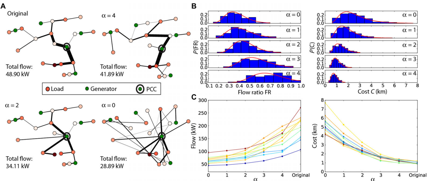
Fig. 4. (A) Example microgrid and the resulting optimized topologies for different rewiring parameters \alpha . Darker shade of red denotes higher load. (B) Distributions of flow ratio and cost for different values of \alpha over all microgrids in Cambridge. The solid red lines indicate the lognormal fits. (C) Total flow and cost with respect to different values of \alpha for the 10 largest microgrids in Cambridge.
