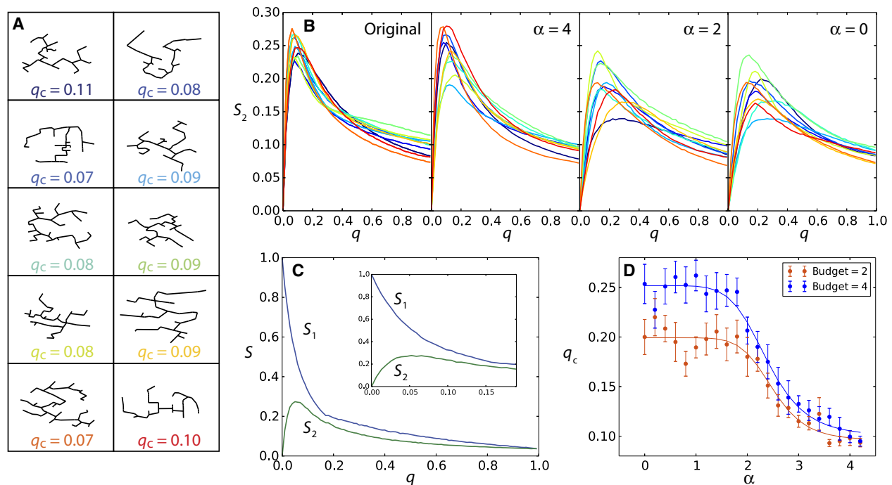
Fig. 5. (A) Topologies and q_c values of the 10 largest microgrids in Cambridge, MA. (B) Size of the second largest connected component S_2 with respect to q for different values of \alpha . The microgrids are color-coded according to (A). (C) Size of the largest and second largest connected component, S_1 and S_2 , respectively, as a function of q for a sample synthetic microgrid of size N = 50 . (D) Percolation threshold q_c as a function of \alpha for ensembles of synthetic microgrids of size N = 50 , averaged over 20 realizations. The solid lines follow Eq. 6.
