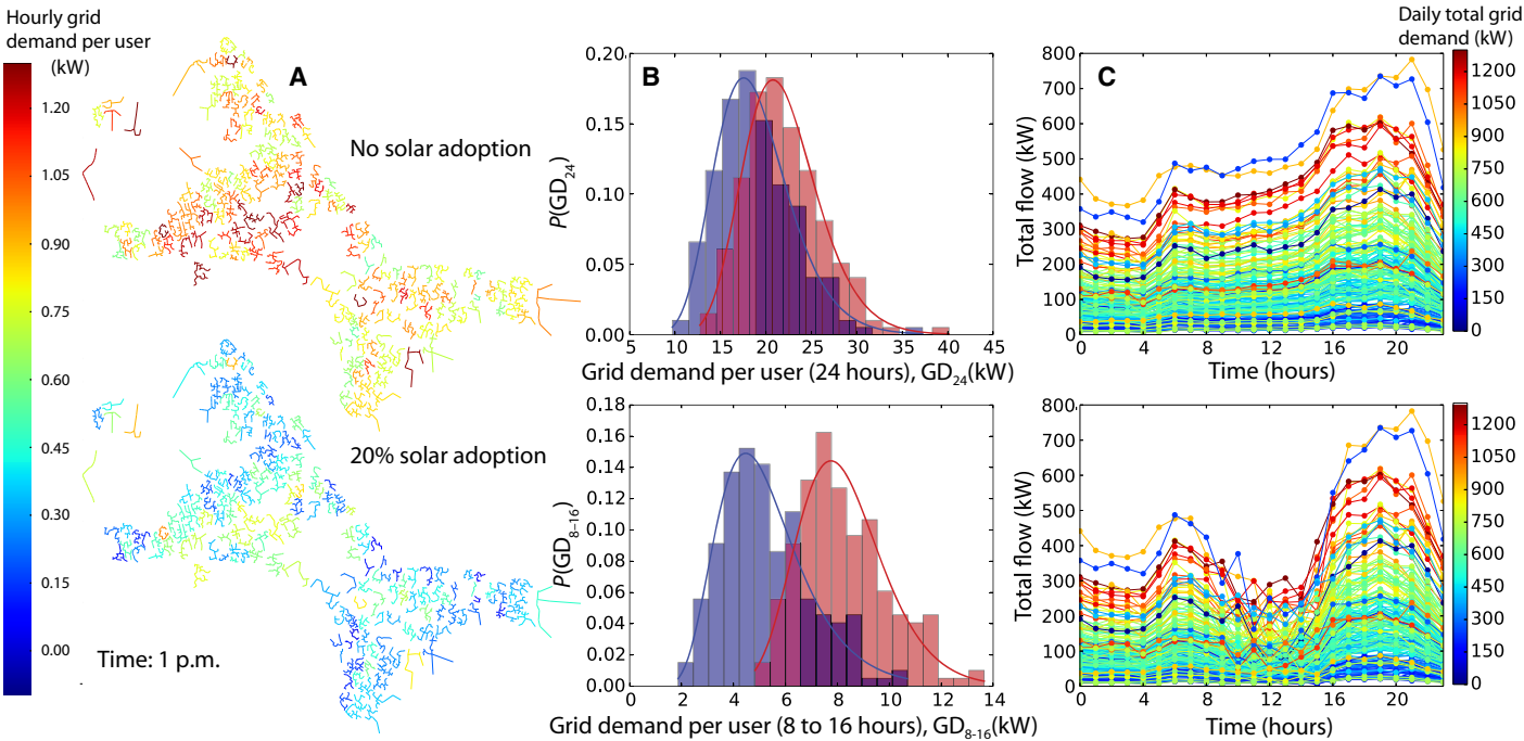
Fig. 3. (A) Proposed microgrids in Cambridge. The colors denote the grid demand per user in the microgrid at 1 p.m. for the no-solar adoption (top) and the 20% solar adoption (bottom) case. (B) Distributions of grid demand for the 200 microgrids for the whole day (top) and daylight hours (bottom) for the no-adoption (red) and the 20% adoption (blue) case. The red and blue solid lines indicate the lognormal fits for the no-adoption and 20% adoption cases, respectively. (C) Total flow in the microgrid as a function of time of day for no solar adoption (top) and 20% solar adoption (bottom). The colors denote the total daily grid demand of each microgrid.
